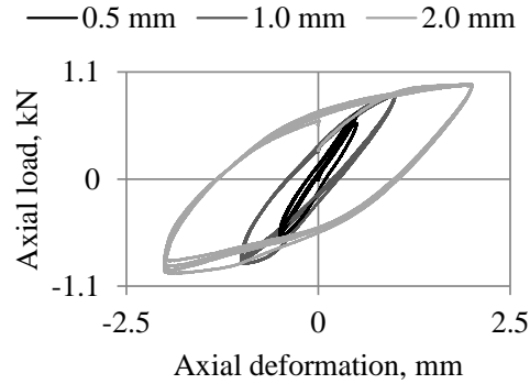
Figure 4. Experimental response of an isolated BRB under cyclic loads
